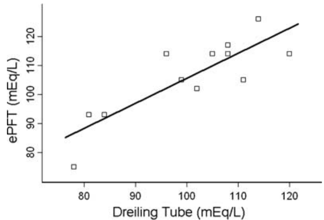
Figure 4. Scatterplot of peak [HCO 3 - ] obtained by the ePFT and DT methods. An excellent correlation was observed between the two methods ( R^2 = 0.84, p < 0.001 ).
